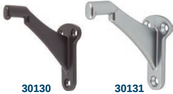
30130 30131 Wall to tip projection: 3-1/4" Wall to center line: 2-1/16"
